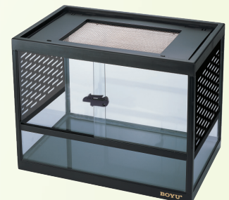
CWG-500T 500x300x380mm
