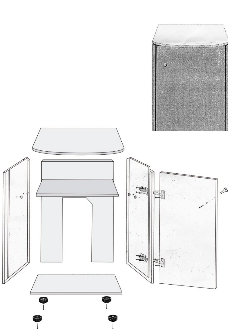
Despiece HS60-AZ
